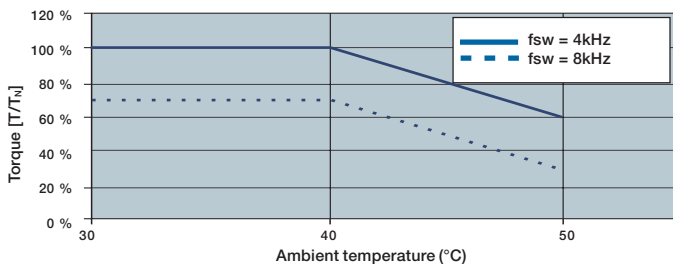
Derating with temperature
